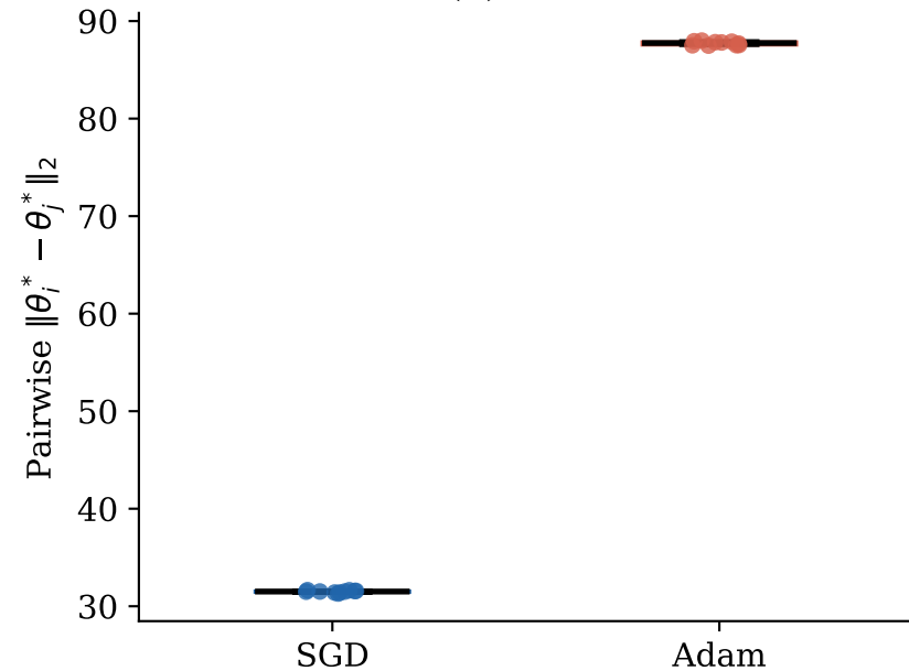
(a) MLP
