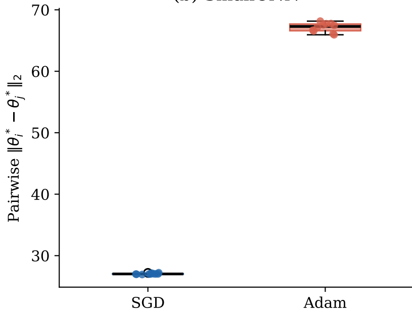
(b) SmallCNN
